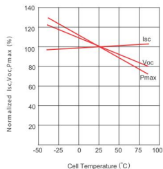
Temperature Dependence of Isc, Voc, Pmax
