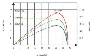
Current-Voltage/Power-Voltage Curve (280W)
